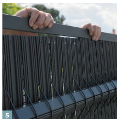
5 Fasten the cap rail at the top of the panel with the flat side on the side of the fold of the panel to secure the slats.
