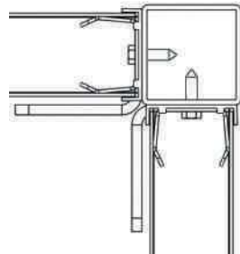
Surface-mounted angle post
