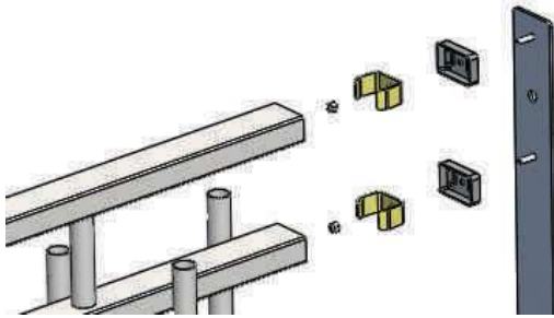
Wall bracket
