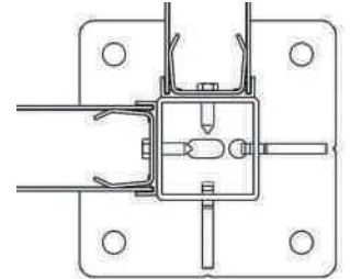
Angle base plate
